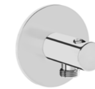
Origin hand shower outlet and holder Chrome £132 - A42625 Brushed Nickel £196 - A4262534 Copper £157 - A4262526 Matt Black £196 - A4262536 Gold £157 - A4262523 H: 90mm P: 75mm
