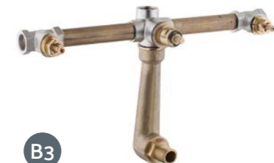
Concealed part for bath/shower mixer £91 - A40834
