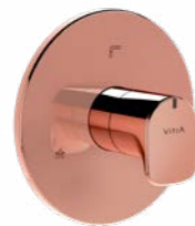
Root built-in diverter, 3-way, round Copper £170 - A4269626 Chrome £140 - A42696 Brushed Nickel £220 - A4269634 Gold £220 - A4269623 H: 170mm P: 80mm
