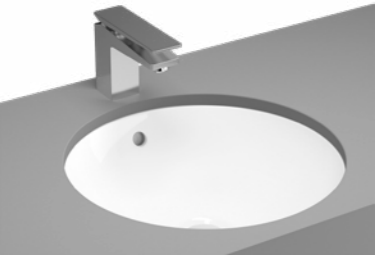
Undercounter washbasin, 0TH, 45cm £200 With overflow hole – 5940B003-1082 Without overflow hole – 5940B003-1083 H: 165mm W: 445mm P: 445mm
