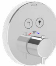
Aquacontrol concealed thermostatic bath mixer, round Chrome £210 – A42718 H: 170mm P: 20mm
