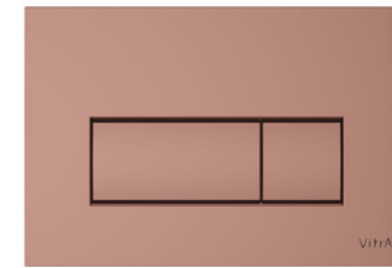
Loop Square mechanical flush plate compatible with all frames Soft Copper £70 - 740-2340 H: 165mm W: 244mm P: 9mm
